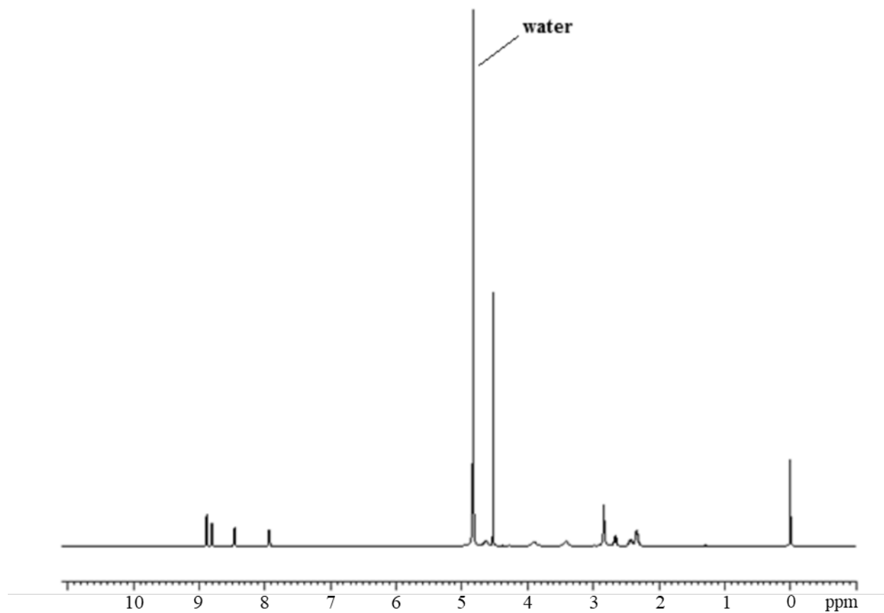
Figure A-2. ^1\text{H} Nuclear Magnetic Resonance Spectrum of Nicotine Bitartrate Dihydrate
