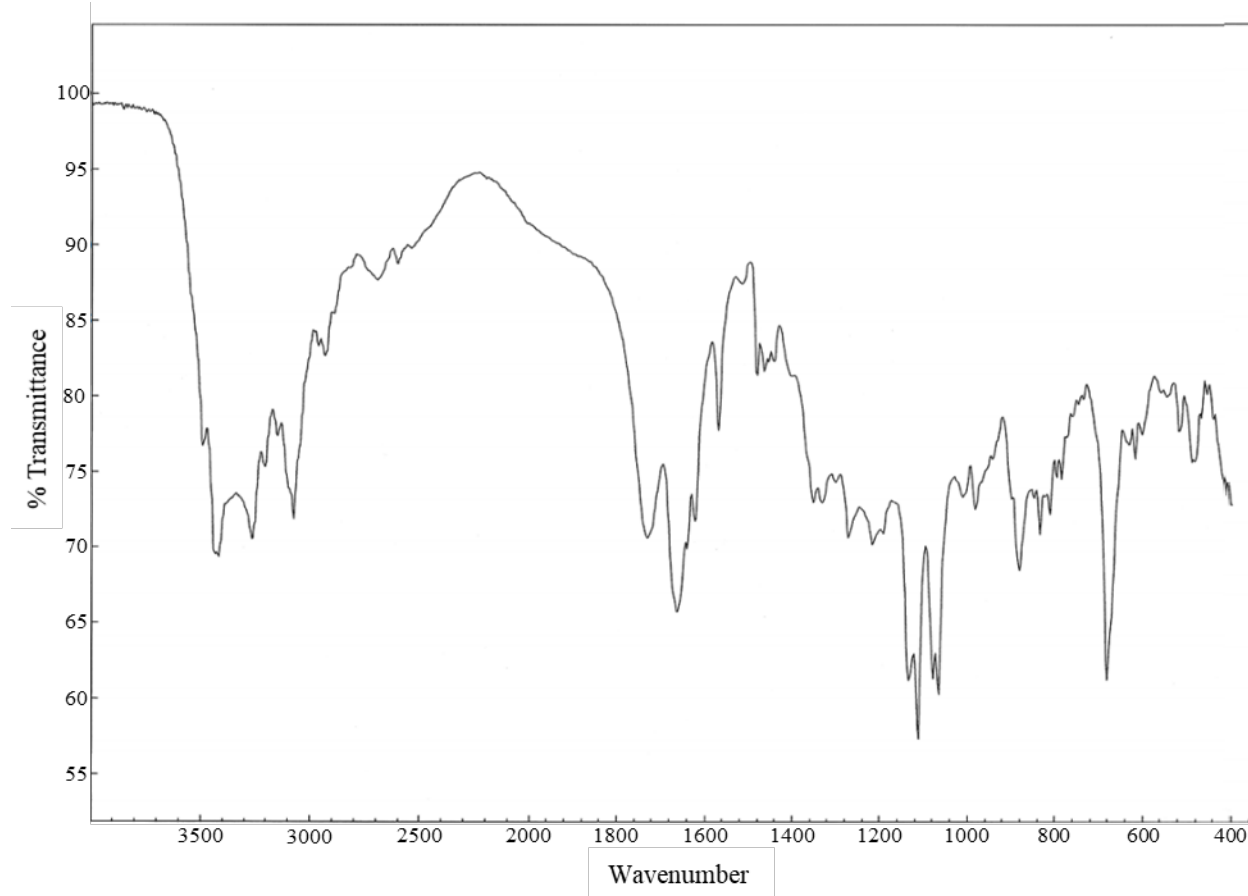
Figure A-1. Infrared Absorption Spectrum of Nicotine Bitartrate Dihydrate
