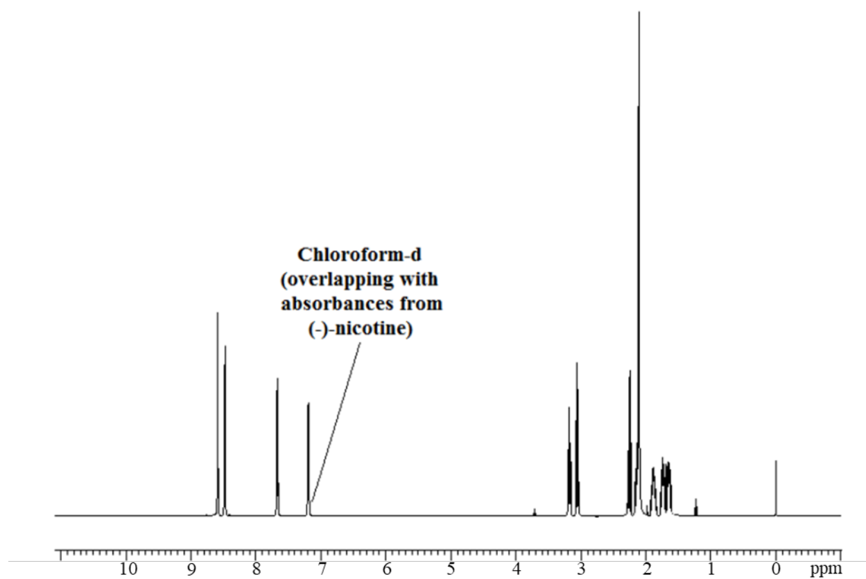
Figure A-5. ^1\text{H} Nuclear Magnetic Resonance Spectrum of Freebase (-)-Nicotine
