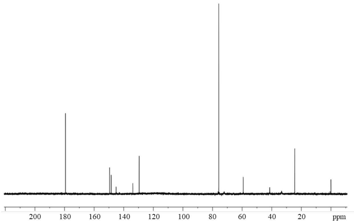
Figure A-3. ^{13}\text{C} Nuclear Magnetic Resonance Spectrum of Nicotine Bitartrate Dihydrate
