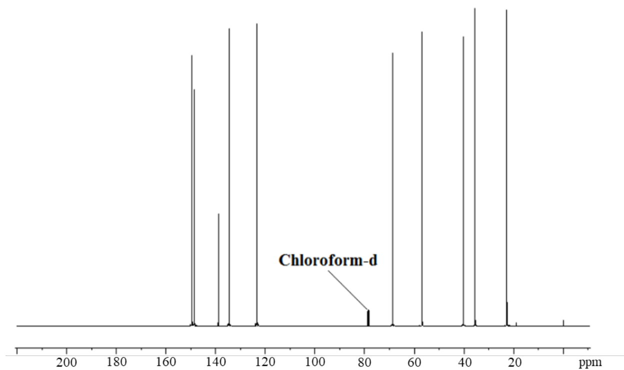
Figure A-6. ^{13}\text{C} Nuclear Magnetic Resonance Spectrum of Freebase (-)-Nicotine
