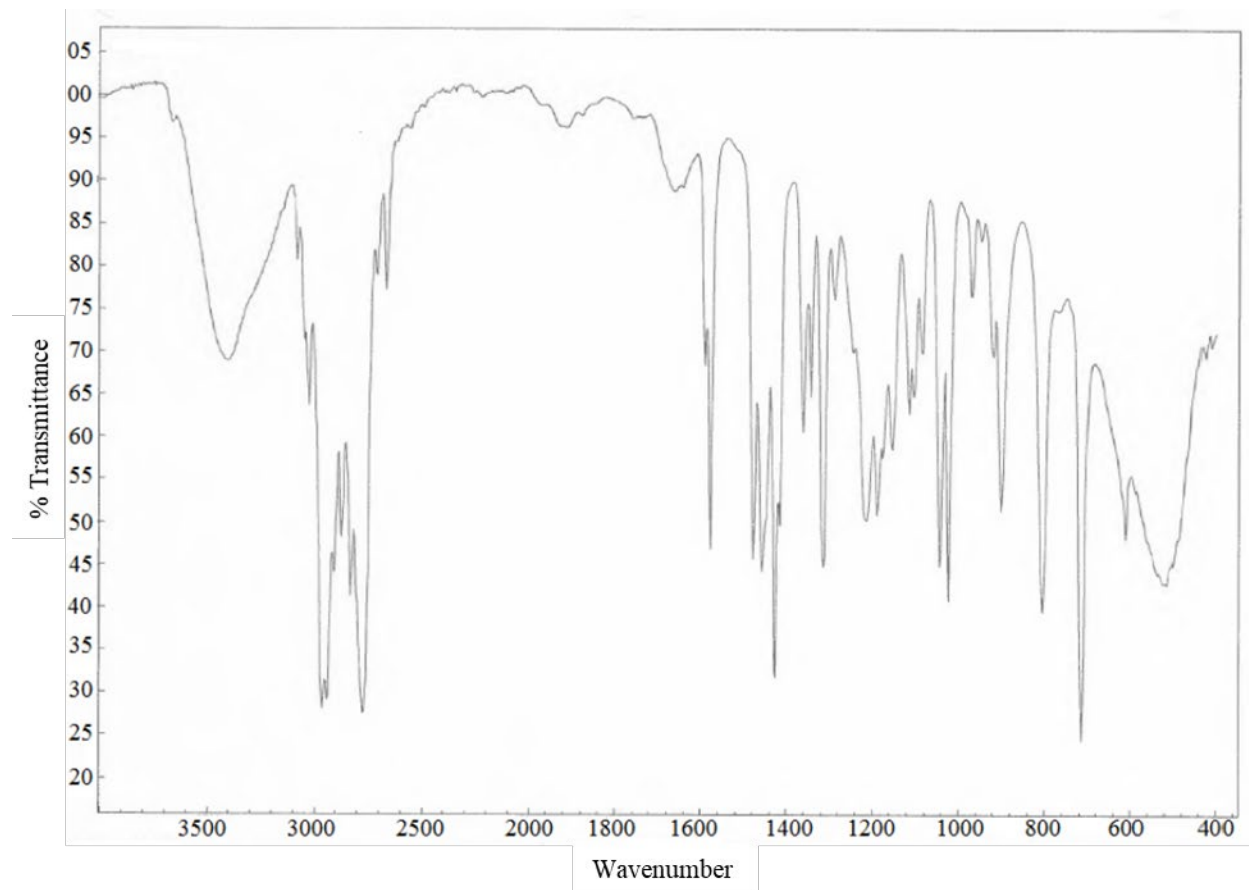
Figure A-4. Infrared Absorption Spectrum of Freebase (-)-Nicotine
